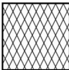
G 3 19 x 19 Outer Tube Frame Wire Diameter 5mm Aperture 50 x 100
