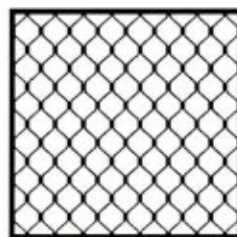
G 4 19 x 19 Outer Tube Frame Wire Diameter 5mm Aperture 56 x 65
